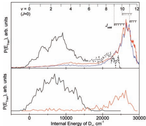
Figure 2. (Top) Internal energies of \text{D}_2 cofragment inferred from the velocity map images of CO in the rotational level J'' = 23 (blue line), 28 (red line), and 55 (black line). (Bottom) Internal energies of \text{D}_2 predicted using QCT calculations to correlate with CO in the rotational levels from J'' = 21 to 25 (red line) and from J'' = 53 to 57 (black line).
