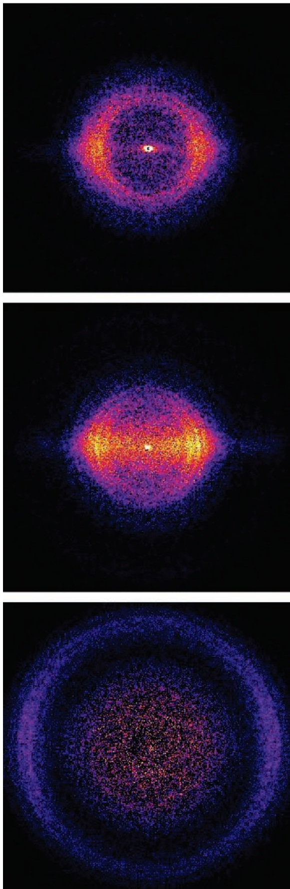
Figure 1. DC sliced velocity map images of CO fragments in several degrees of rotational excitation: J'' = 23, 28, and 55 from the 327 nm photolysis through the \text{R}_1(1) rotational level of the 2^2_4^3 vibrational band of the S_1 state of \text{D}_2\text{CO} .
